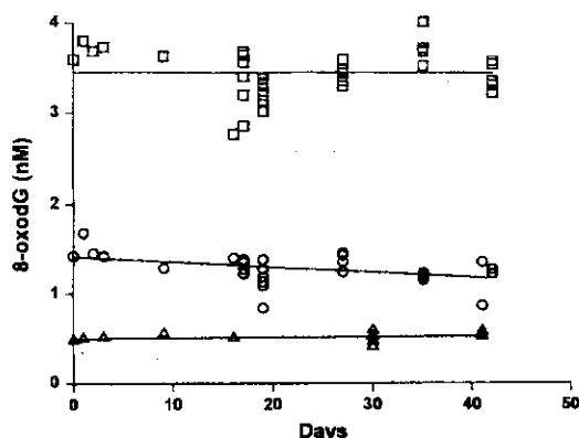
FIGURE 1 Quality control; samples of 8-oxodG solutions A ( \Delta ), B/C ( \circ ) and D ( \square ) were analysed by HPLC with coulometric electrochemical detection over a period of 42 days which included the interval allowed to collaborators for analysis. Lines indicate linear regression for each sample.
