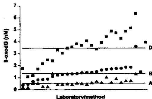
FIGURE 2 Inter-laboratory comparison of 8-oxodG analyses, samples A ( \Delta ), B/C ( \circ ), D ( \square ). The order of laboratories/methods on the x-axis is determined by the order of values reported for sample B/C. Horizontal lines for A, B/C and D indicate the mean concentrations as determined by the distributing laboratory.
