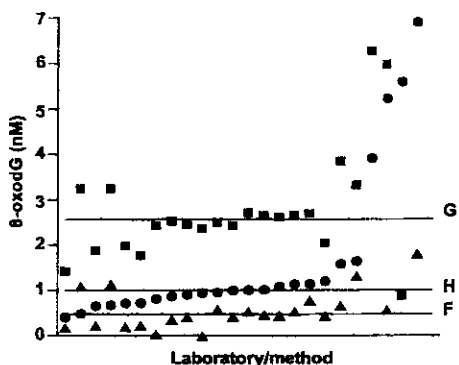
FIGURE 3 Inter-laboratory comparison of 8-oxodG analyses, samples F (▲), E/H (●), G (■). The order of laboratories/methods on the x-axis is determined by the order of values reported for sample E/H. Horizontal lines for F, E/H and G indicate the mean of concentrations as determined in the distributing laboratory.
