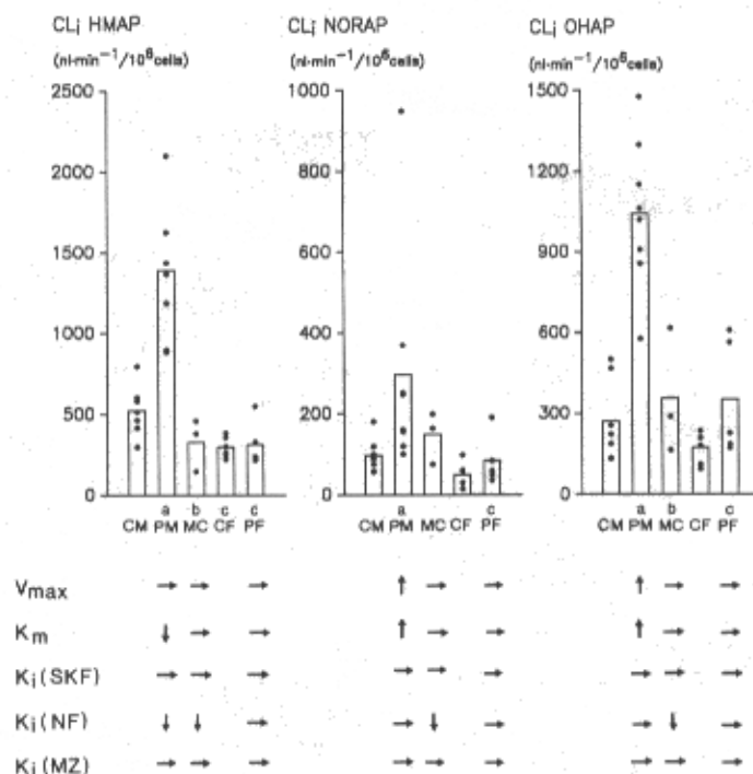
Fig. 4. Individual and average (boxes) values of intrinsic clearance ( CL_i ) of antipyrine to 3-methylhydroxy (HMAP), nor- (NORAP) and 4-hydroxyantipyrine (OHAP) in isolated hepatocytes from male control (CM), phenobarbital pretreated male (PM), 3-methylcholanthrene pretreated male (MC), control female (CF) and phenobarbital pretreated female (PF) Wistar rats. a, b and c indicate significant differences from control values, between the PB and MC group and between the sexes, respectively. The vertical arrows indicate significant changes of Michaelis-Menten constants and competitive inhibition constants ( K_j ) of SKF 525A (SKF), \alpha -naphthoflavone (NF) and antipyrine (MZ), the horizontal arrows indicate lack of significant changes.
