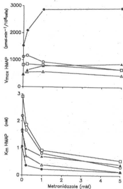
Fig. 5. Effect of increasing concentration of metronidazole on mean V_{max} and K_m for formation of 3-methylhydroxyantipyrine (HMAP) in isolated hepatocytes from male control (○, N = 5); phenobarbital pretreated male (●, N = 5); 3-methylcholanthrene pretreated male (□, N = 3); control female (△, N = 4); and phenobarbital pretreated female (▲, N = 4) Wistar rats.
