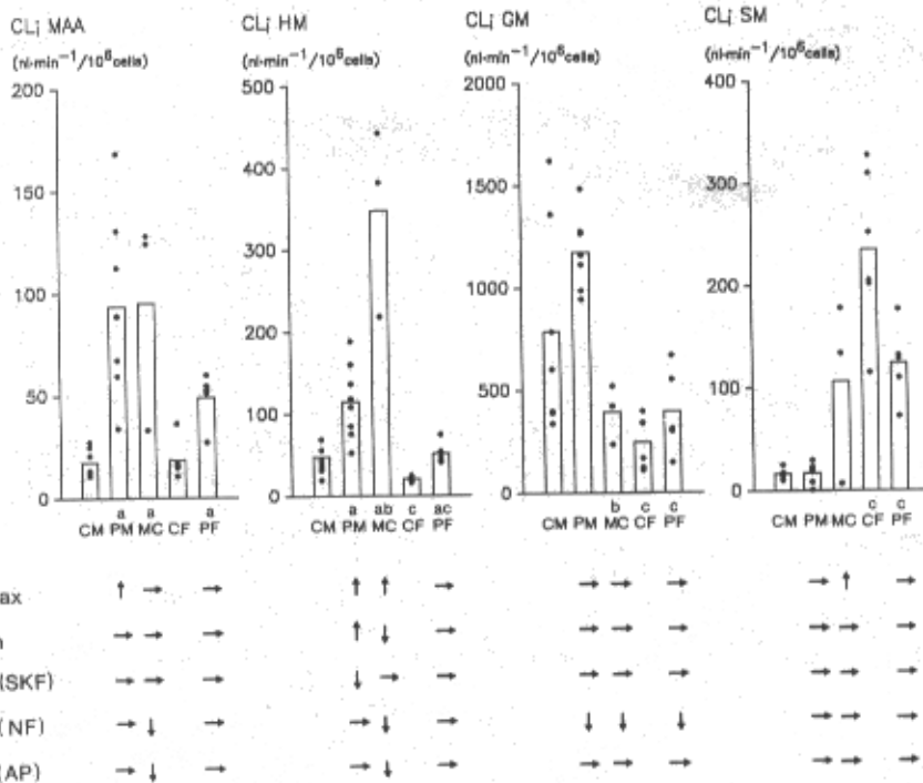
Fig. 3. Individual and average (boxes) values of intrinsic clearance ( CL_i ) of metronidazole to its acetic acid (MAA) and hydroxy (HM) metabolite and glucuronide (GM) and sulphate (SM) conjugate in isolated hepatocytes from male control (CM); phenobarbital pretreated male (PM); 3-methylcholanthrene pretreated male (MC); control female (CF); and phenobarbital pretreated female (PF) Wistar rats: a, b and c indicate significant differences from control values, between the PB and MC group and between the sexes, respectively. The vertical arrows indicate significant changes of Michaelis-Menten constants and competitive inhibition constants ( K_i ) of SKF 525A (SKF), \alpha -naphthoflavone (NF) and antipyrine (AP), the horizontal arrows indicate lack of significant changes.
